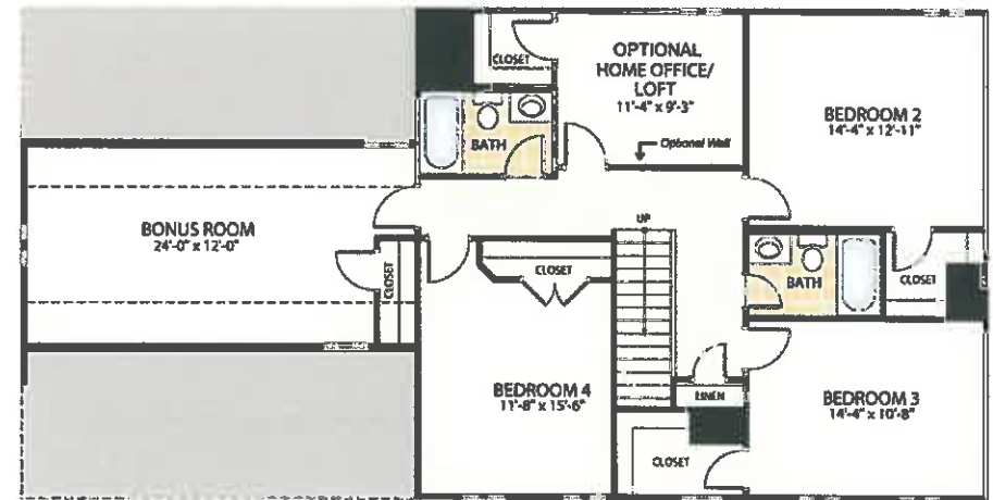
SECOND FLOOR PLAN ELEVATION
